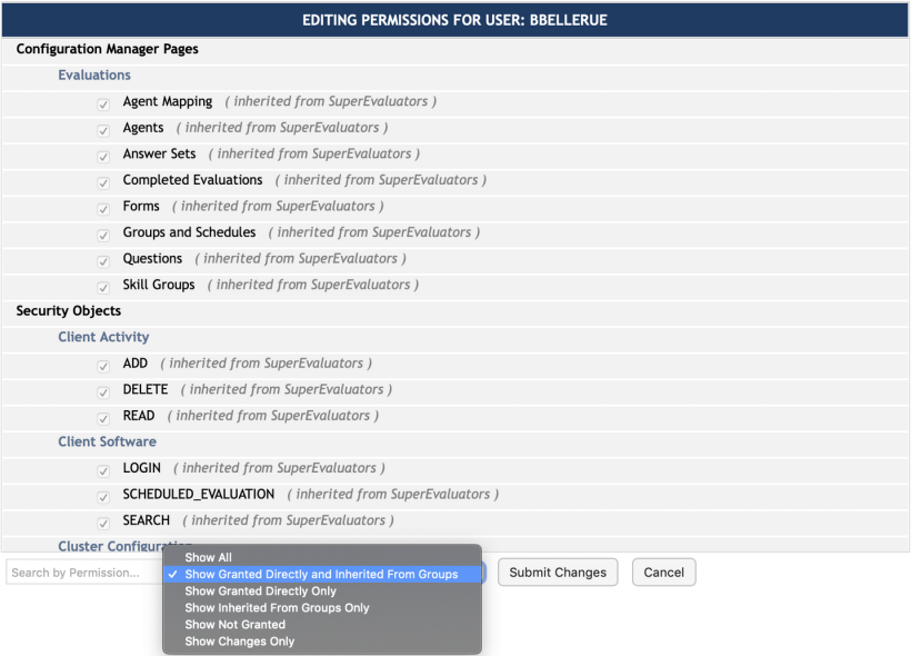
Fig. 7.99 Permissions with Filter Set to Show Granted Directly And Inherited From Groups
