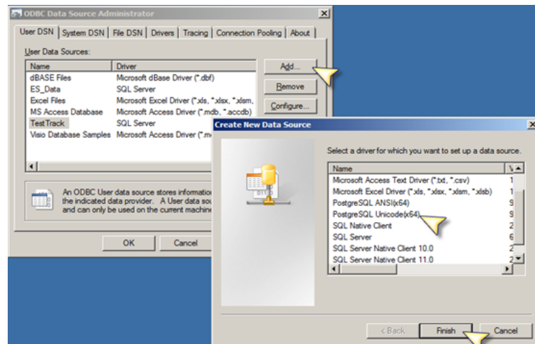
Fig. 4.2 Add PostgreSQL Connector
