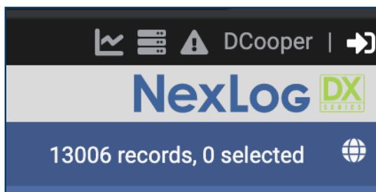
Fig. 12.16 Reports Icon
