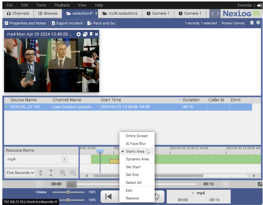
Fig. 4.27 Static Area
