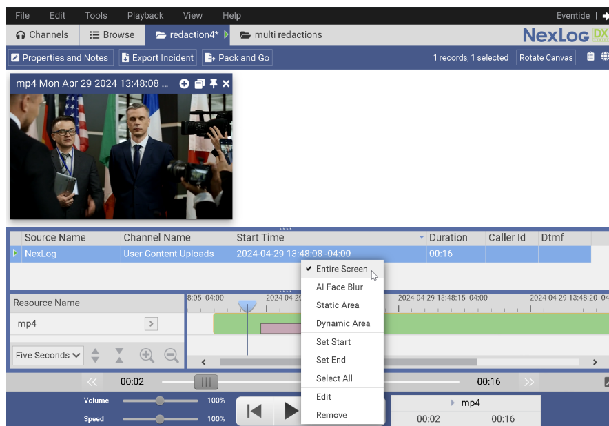
Fig. 4.16 Entire Screen
