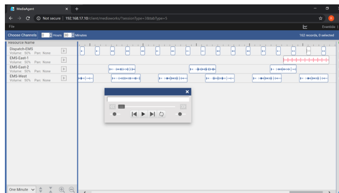
Fig. 17.8 Timeline Only
