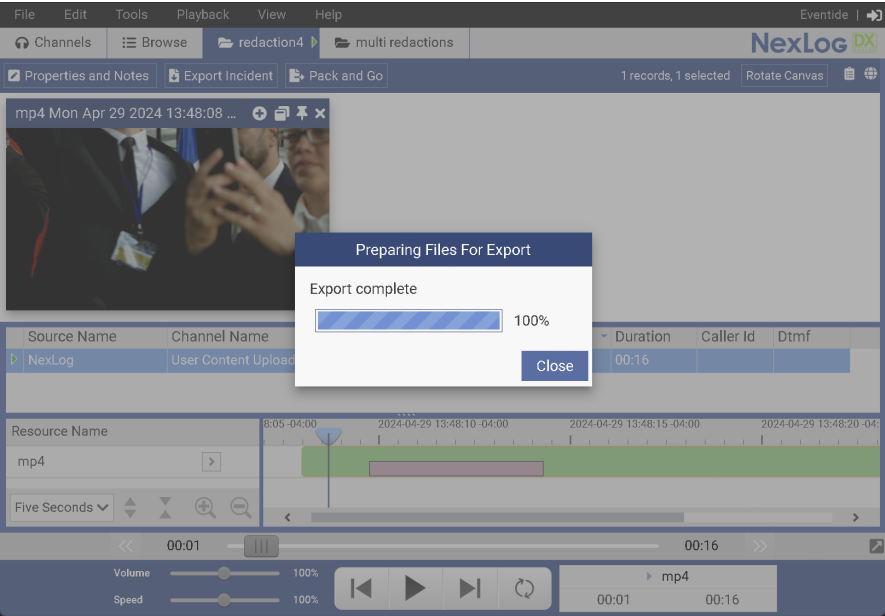
Fig. 4.19 Redaction Complete
