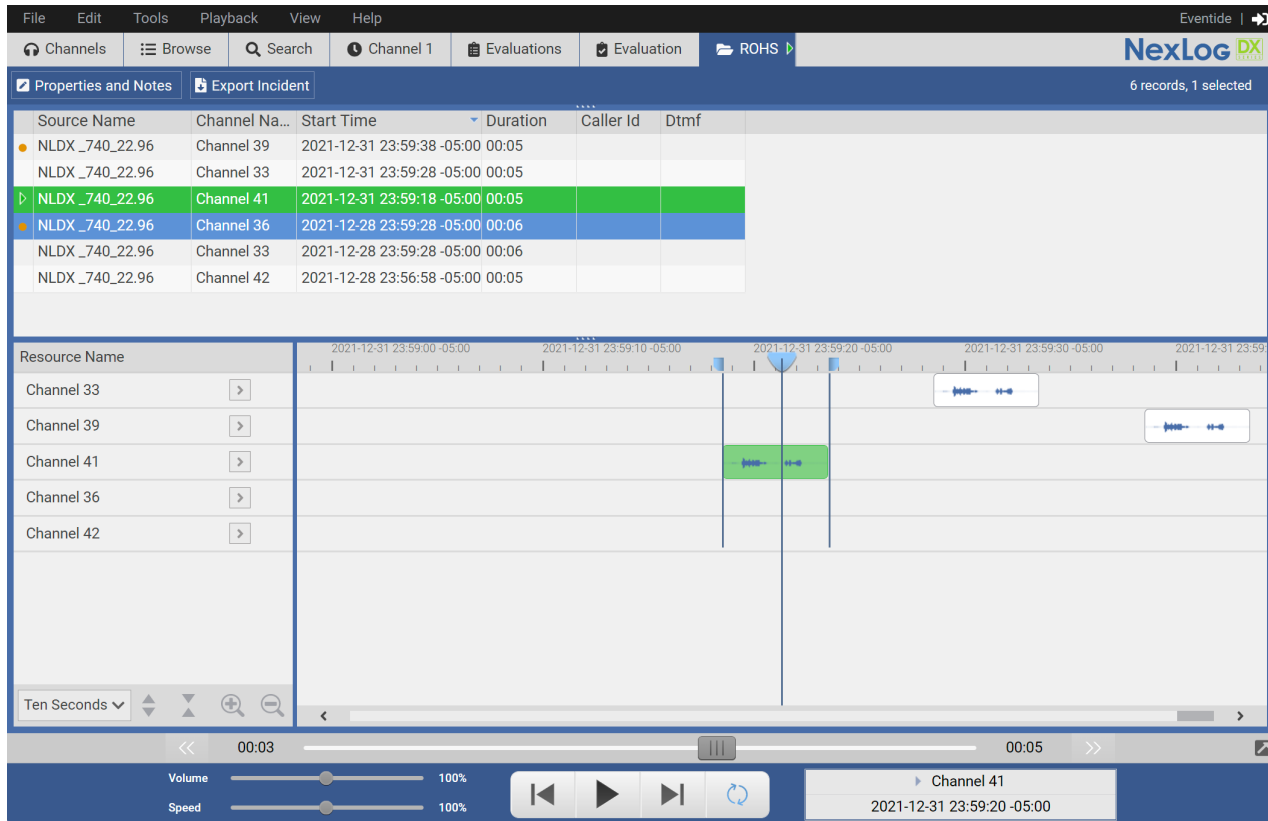
Fig. 13.11 Light Mode
