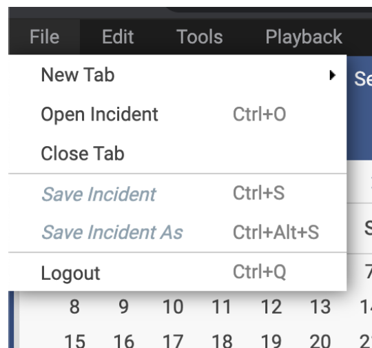
Fig. 13.3 File Menu
