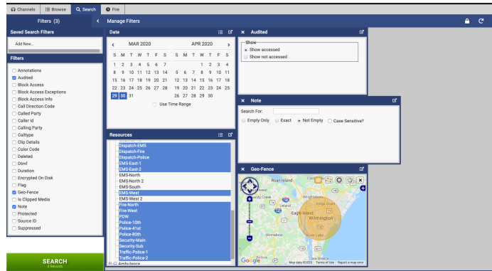
Fig. 2.7 Expanded Search
