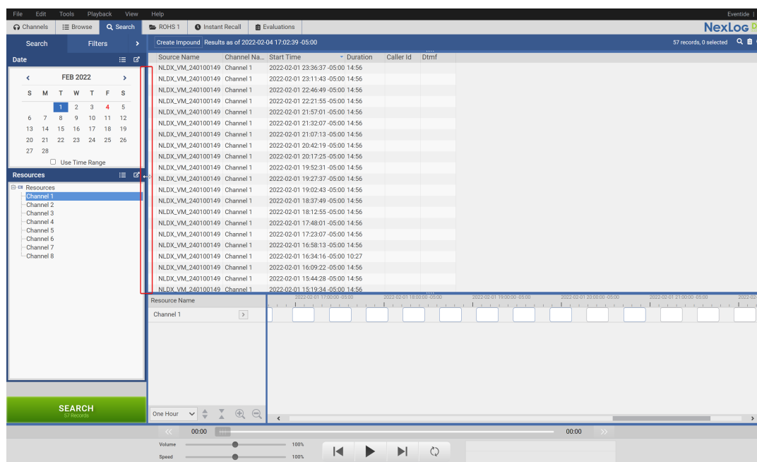
Fig. 3.21 Standard View
