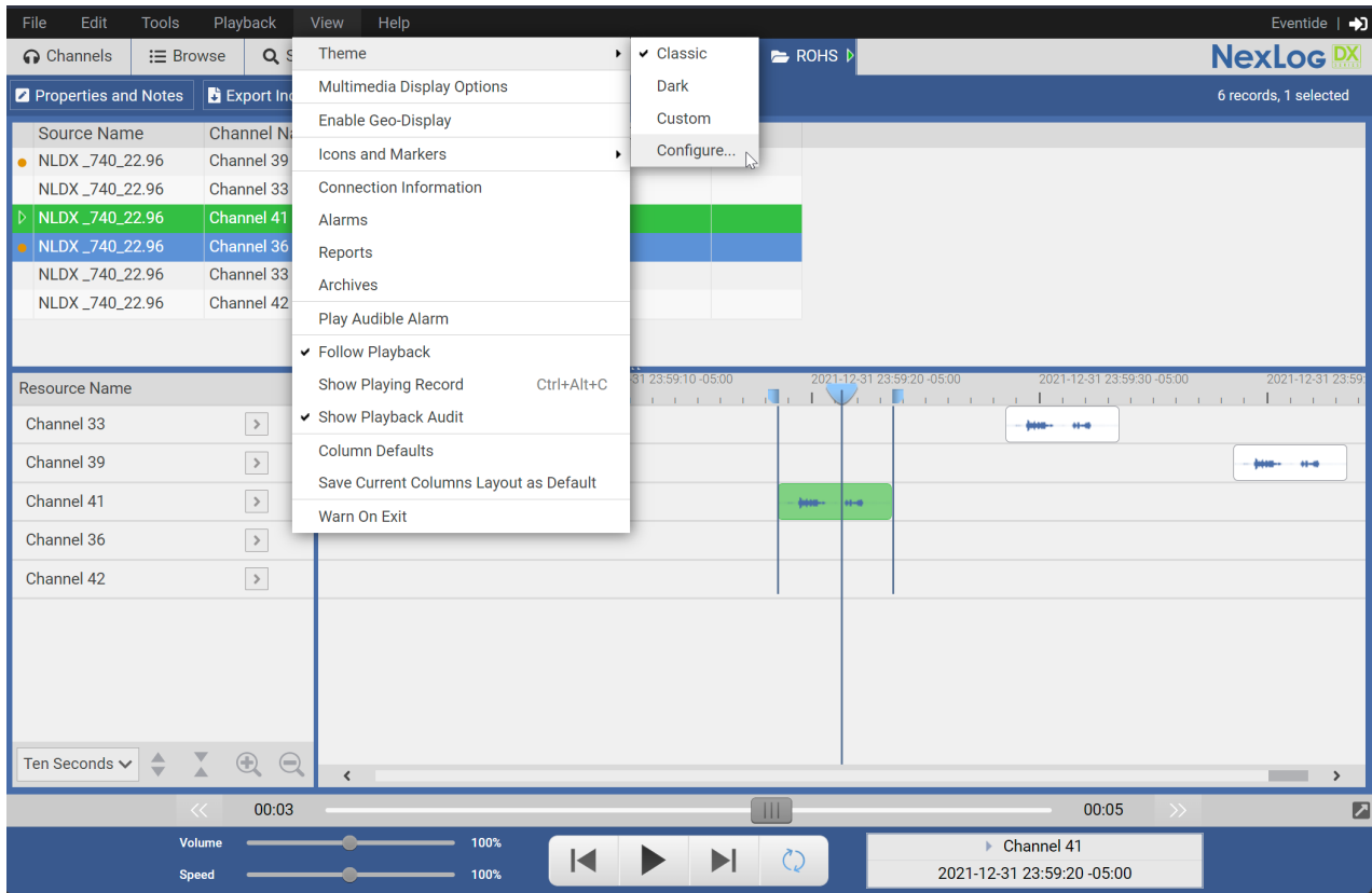
Fig. 13.12 Theme Configure
