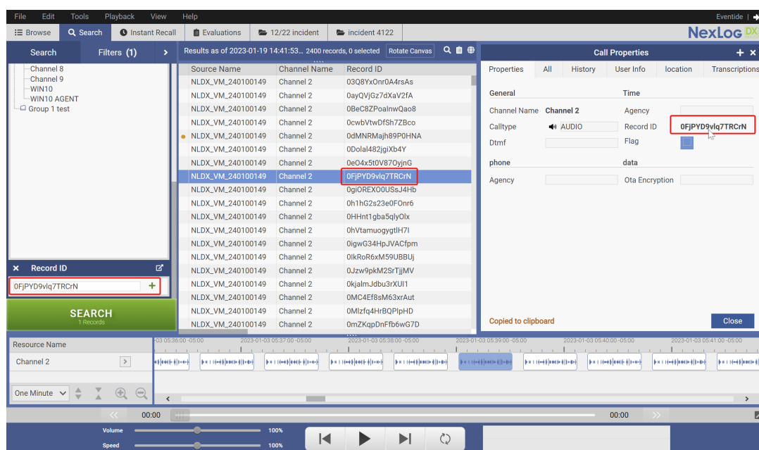
Fig. 2.4 Record ID
