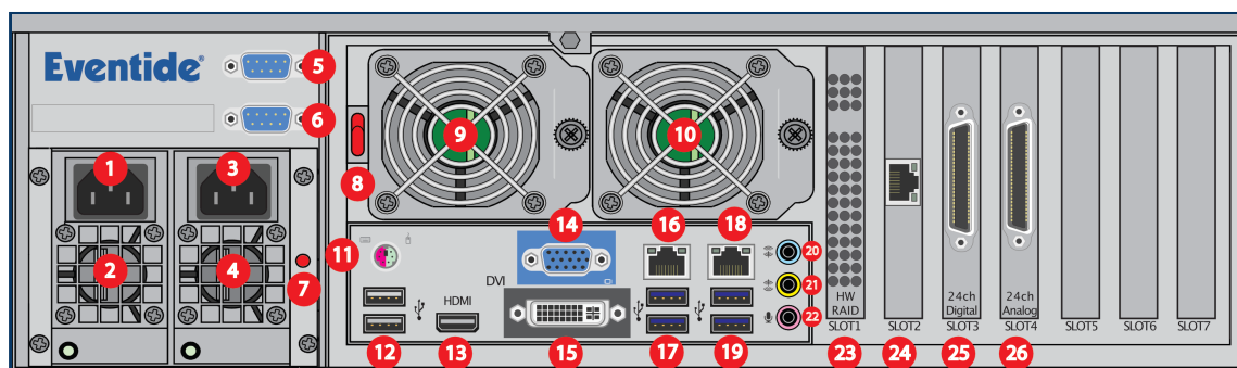
Fig. 2.9 Diagram of NexLog 740 DX-Series™ Recorder Rear Panel
