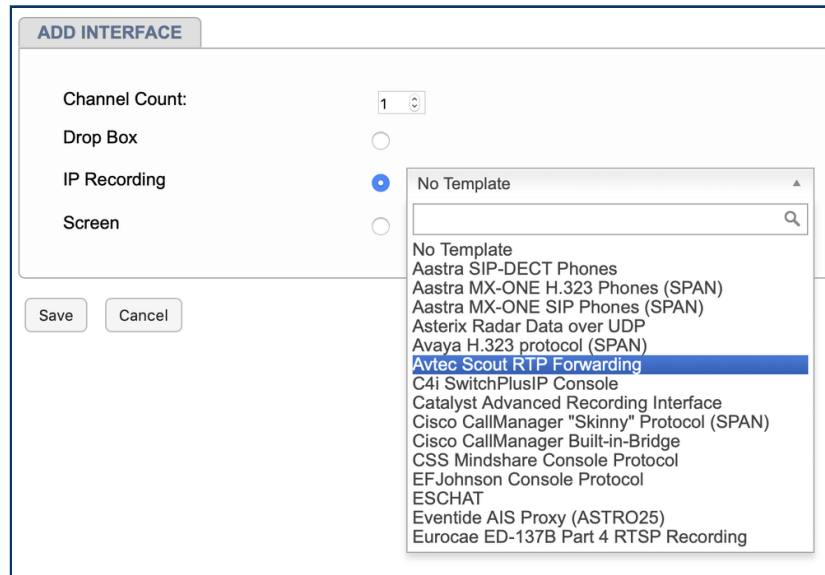
Fig. 11.1 IP Recording Virtual Interface Template Menu
