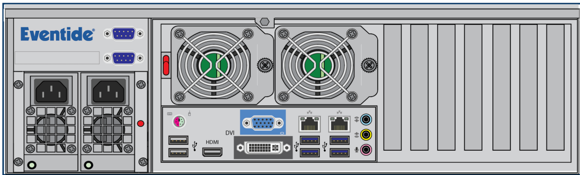
Fig. 2.8 Typical NexLog 740 DX-Series™ Recorder Rear Panel
