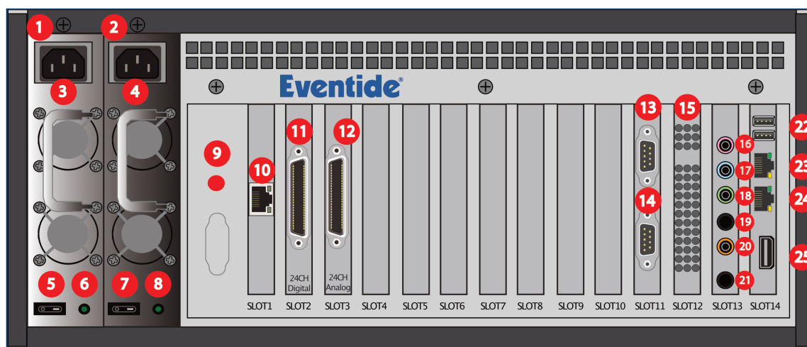
Fig. 2.10 Typical NexLog 840 DX-Series™ Recorder Rear Panel
