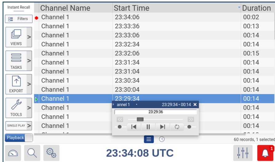
Fig. 5.4 Recall Screen Results with Transport Pop Up
