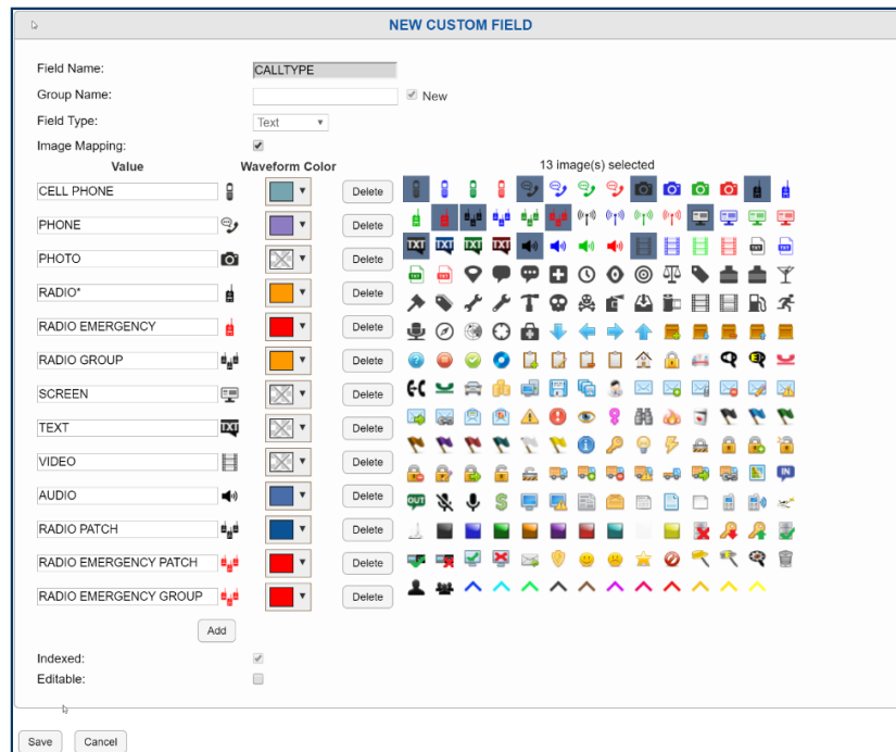
Fig. 6.34 Calltype Field Configuration
