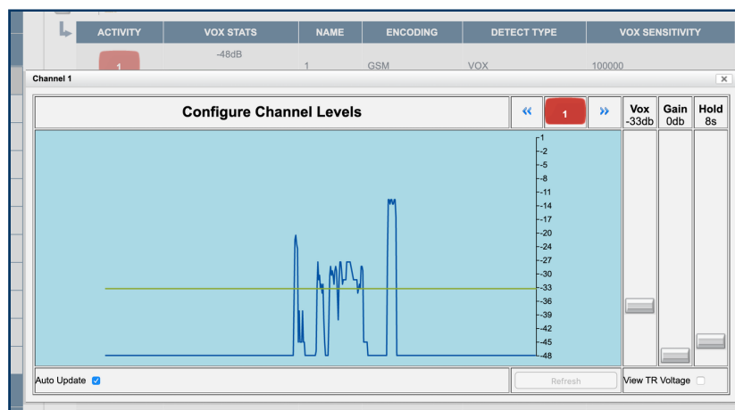
Fig. 6.19 Recording Interfaces Detail Level Graph
