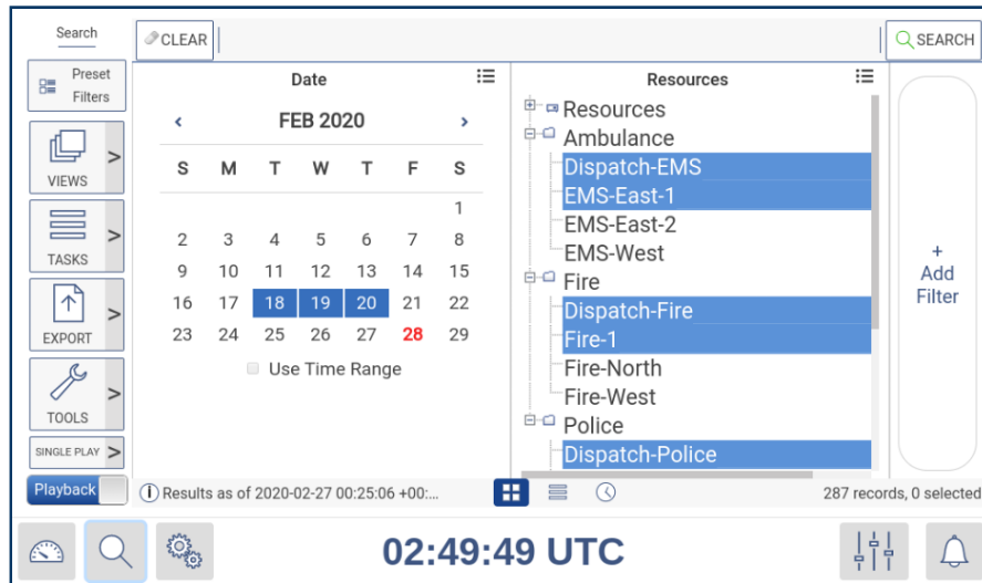
Fig. 5.3 Front Panel Replay Screen, showing Calendar Mode
