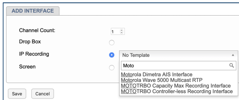
Fig. 11.2 IP Recording Virtual Interface Template Menu With Search Input
