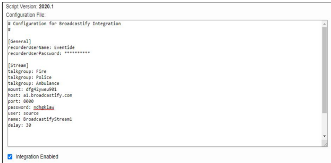
Fig. 7.53 Broadcastify Configuration
