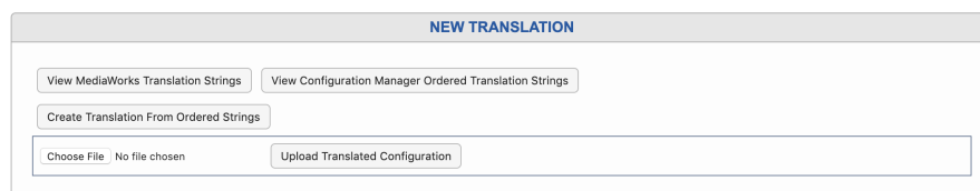
Fig. 7.11 New Translations
