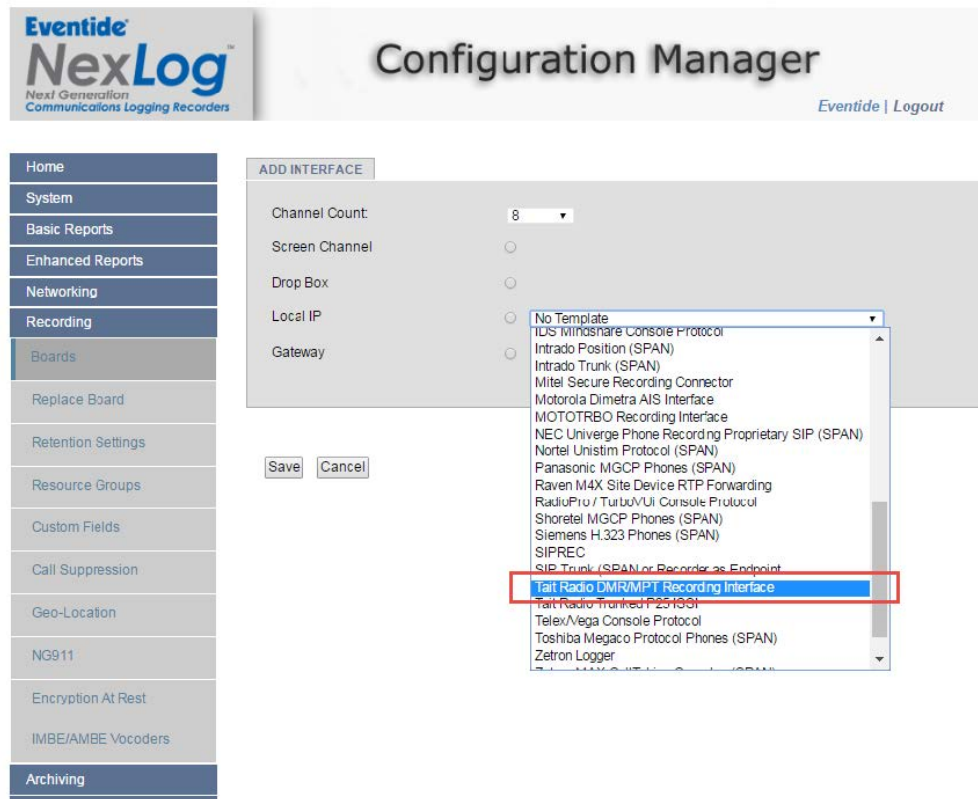
Fig. 6.126 Select Interface
