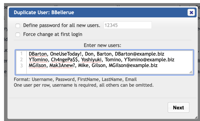
Fig. 7.97 Duplicate User
