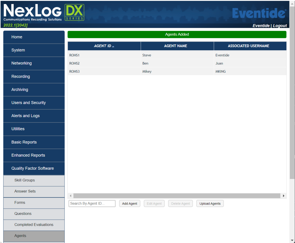
Fig. 7.147 Agents Added
