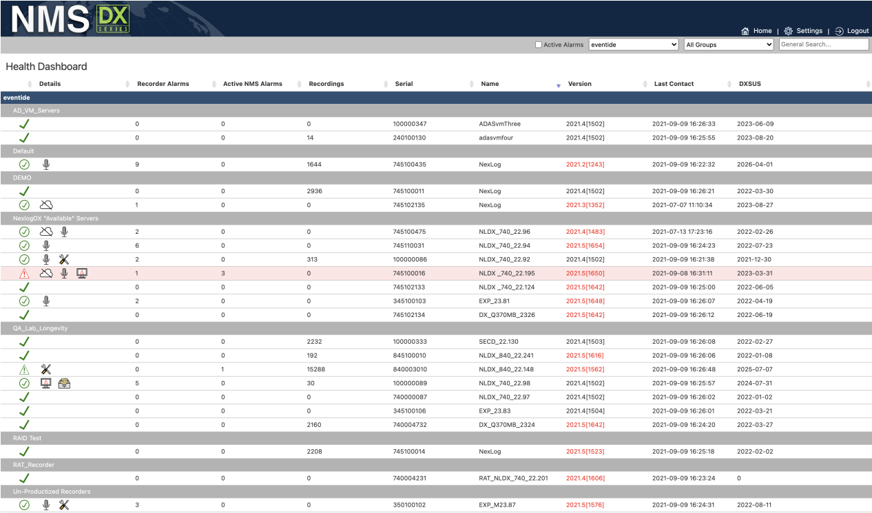
Fig. 7.136 NMS Dashboard
