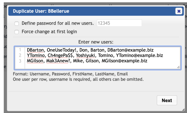
Fig. 7.112 Duplicate User
