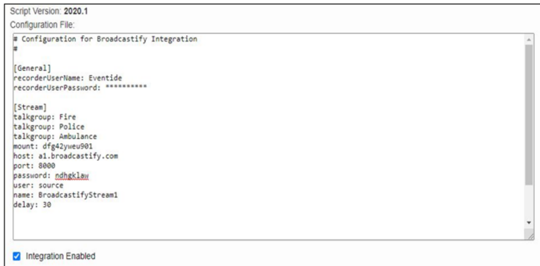
Fig. 7.54 Broadcastify Configuration
